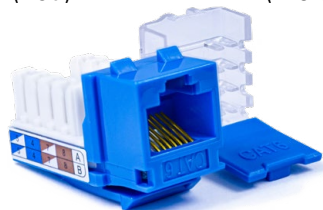
SC-CAT6J-BL (Blue)
